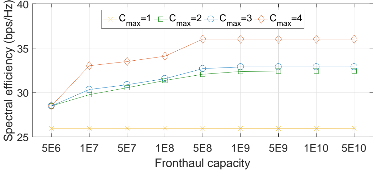
Figure 4.8: Impacts of different C_{max} values and fronthaul capacity
