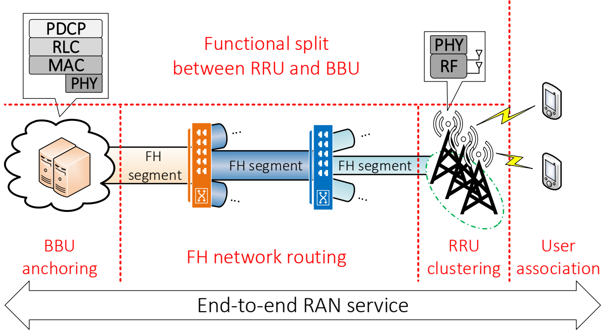
Figure 4.1: Five design issues of C-RAN to deliver the E2E RAN service
