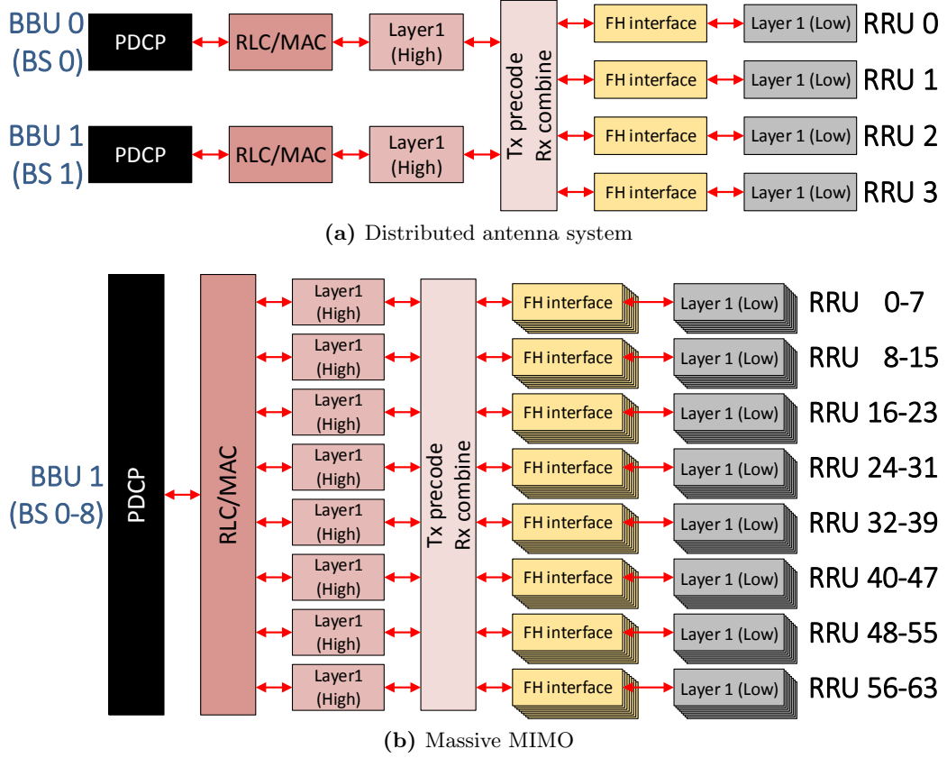
Figure 3.3: Two C-RAN deployment examples
