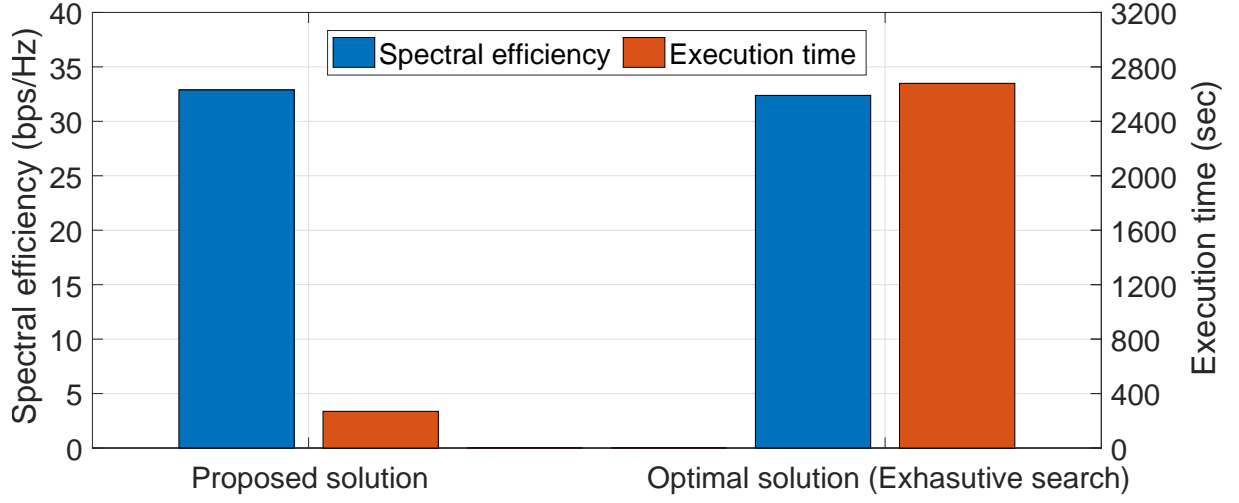
Figure 4.6: Comparison between proposed/optimal solutions
