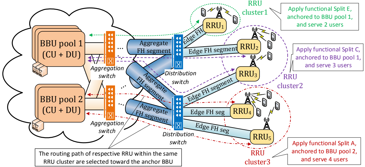
Figure 4.2: C-RAN topology example with three formed RRU clusters
