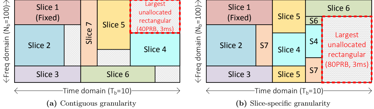
Figure 5.12: Examples of radio resource partitioning
