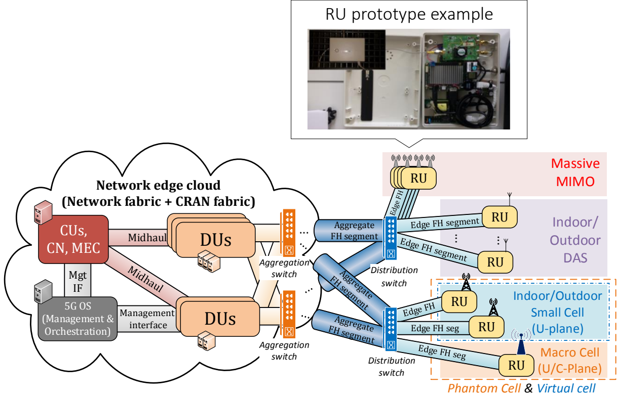
Figure 8.1: An example of 5G edge cloud deployment
