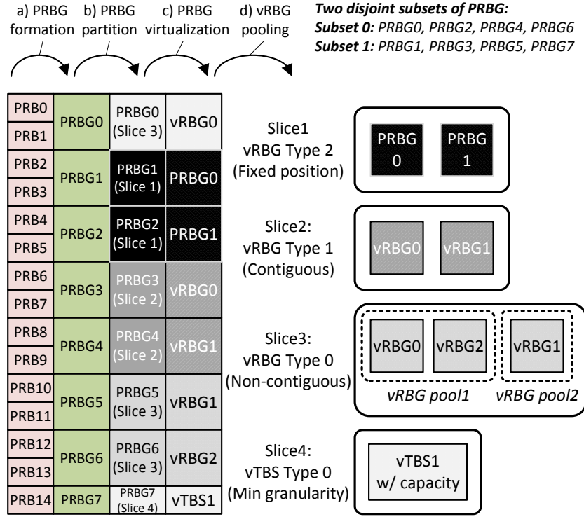
(a) Stages of building vRBG and vRBG pool
