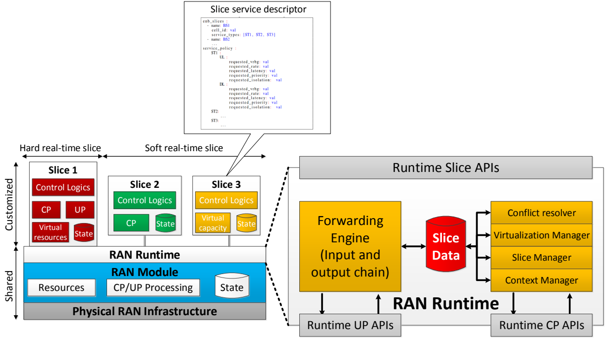
Figure A.12: Architecture de RAN Runtime.
