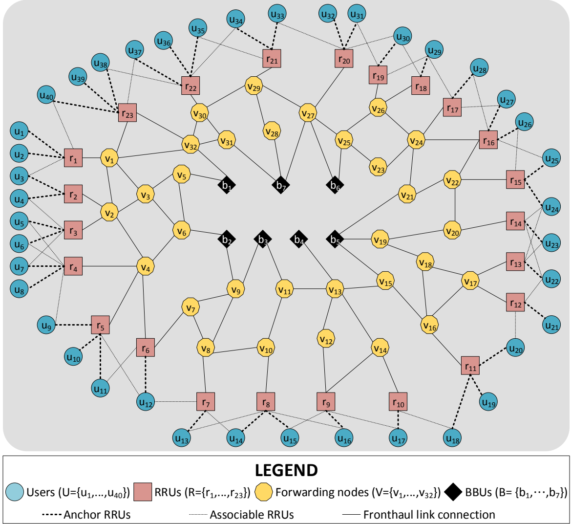
Figure 4.9: Large-scale simulated C-RAN topology
