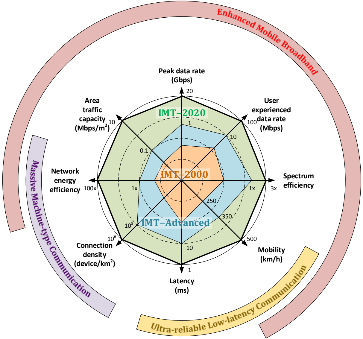
Figure 1.1: IMT-2020 vision on 5G
