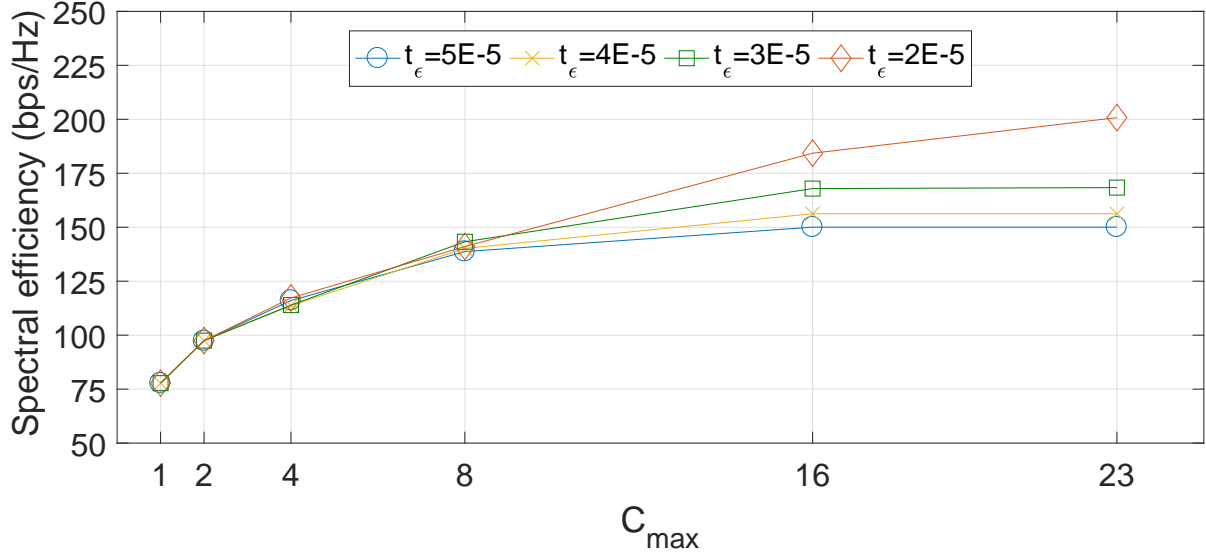
Figure 4.10: Impacts of different C_{max} values and fronthaul delay
