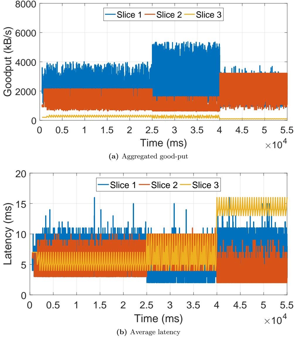
Figure 5.17: Slice performance of dynamic inter-slice resource partitioning
