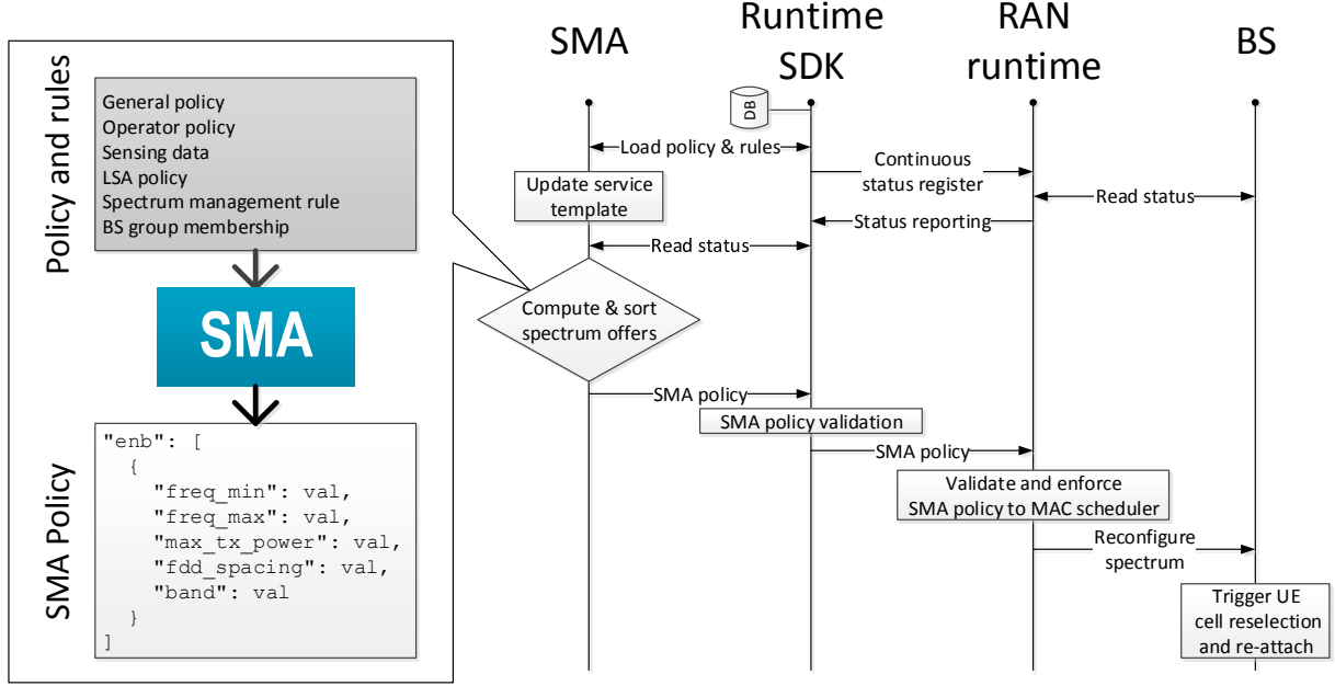
Figure 7.7: Design of spectrum management application
