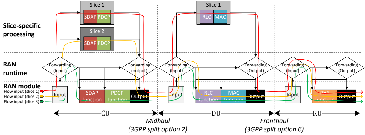
Figure 5.10: UP forwarding paths in three-tier disaggregated RAN (CU, DU, RU)
