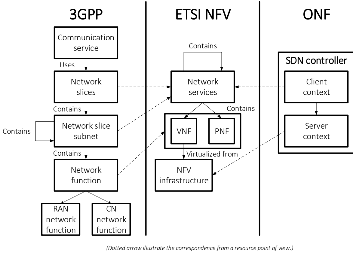
Figure 6.1: Mapping between the slicing information models of 3GPP, ETSI and ONF from [2]
