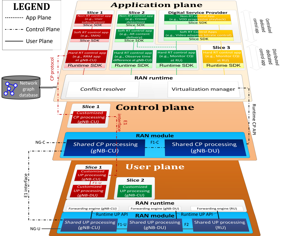
Figure 7.4: SDK and application plane for flexible and programmable RAN control
