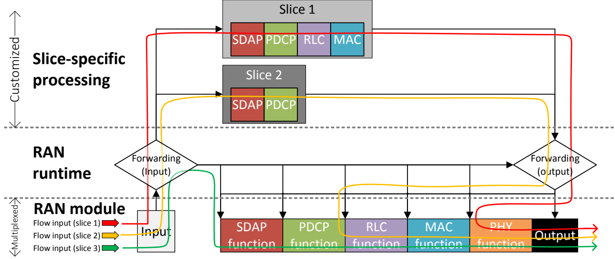
Figure 5.9: Forwarding engine and UP forwarding paths
