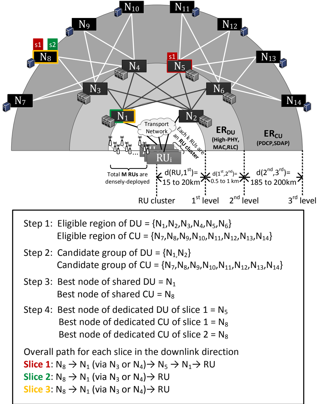
Figure 6.8: Example of a two-stage function placement for multi-service
