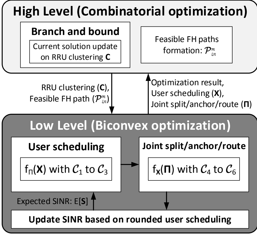
Figure 4.4: Proposed solution of formulated problem
