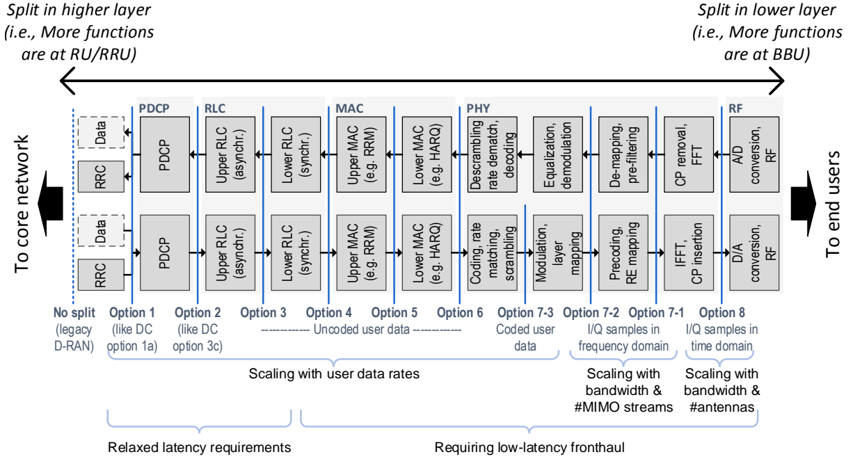
Figure 1.4: Functional split options defined by 3GPP in [1]
