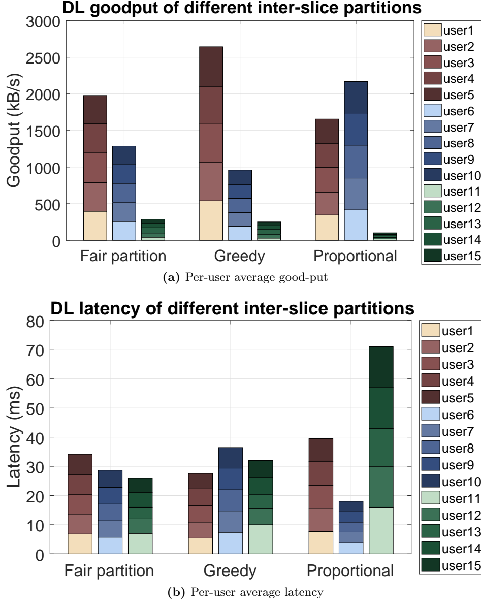
Figure 5.18: User performance of dynamic inter-slice resource partitioning
