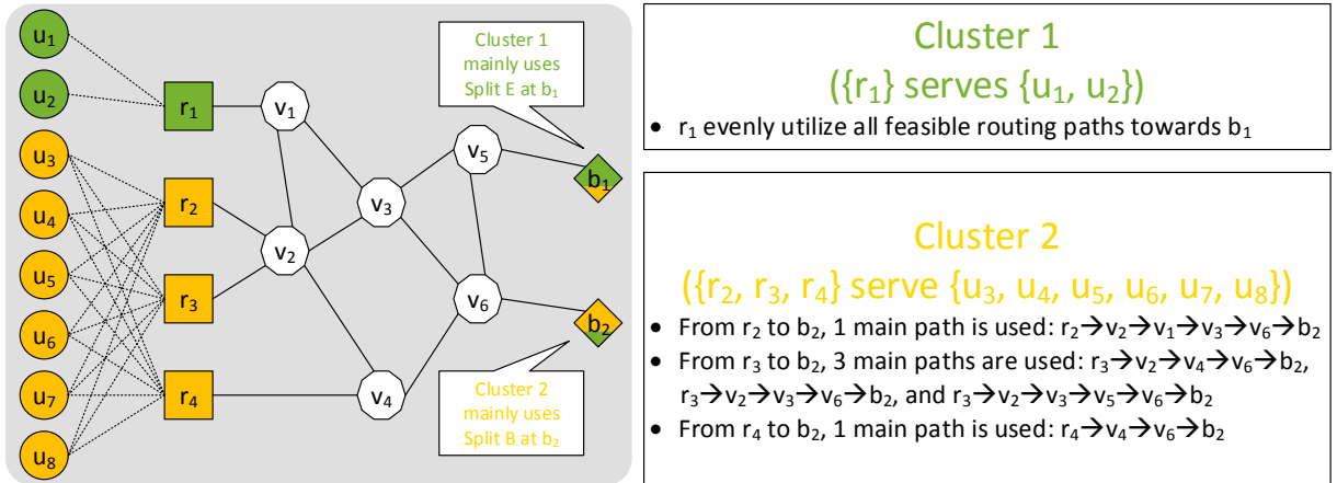
Figure 4.7: Two formed clusters to provide the end-to-end RAN service
