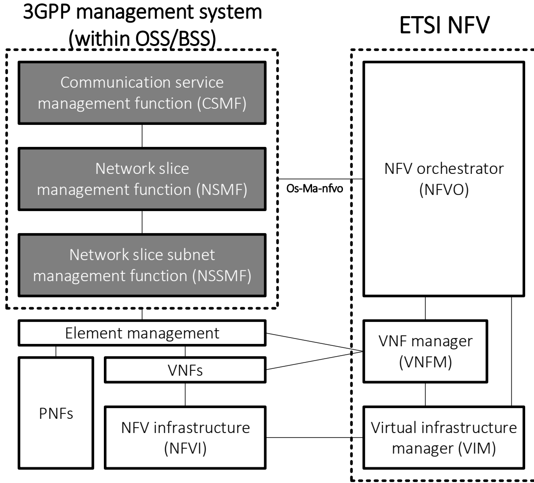
Figure 6.3: 3GPP network slice management in an ETSI NFV architecture from [2]
