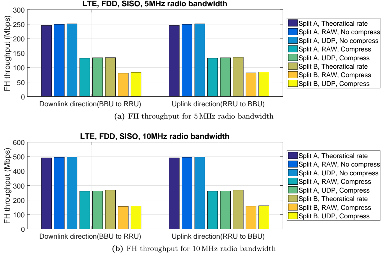
Figure 3.6: FH throughput for 5 MHz and 10 MHz radio bandwidth
