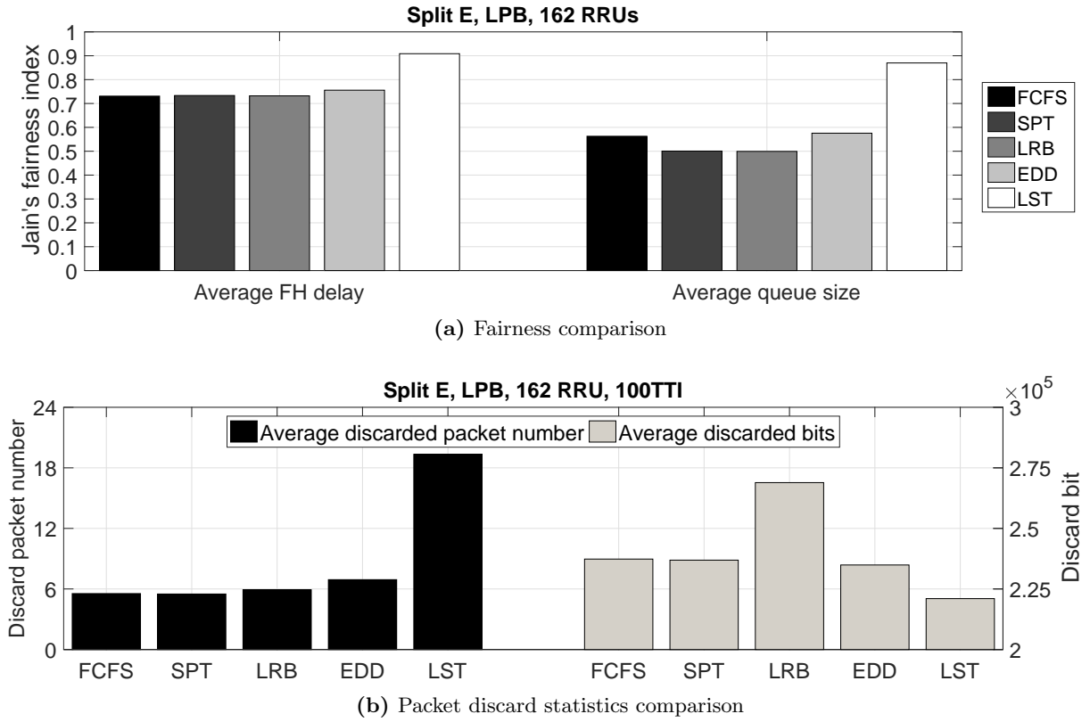
Figure 2.14: Fairness and packet discard statistics among several packet schedule policies
