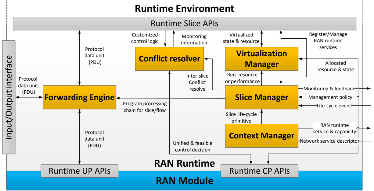
Figure 5.11: Message flows between RAN runtime services
