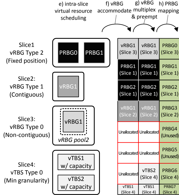
(b) Stages of accommodating vRBG to PRBG
