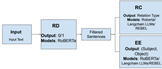
Figure 1: The ERE pipeline workflow
