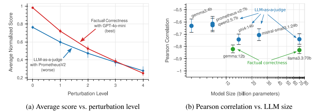
FIGURE 3 – Performance of factuality evaluation methods.
