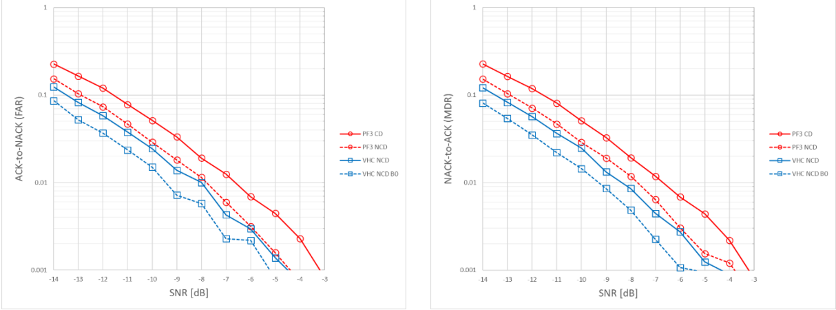
Figure 5: FAR and MDR performance with intra frequency-hopping
