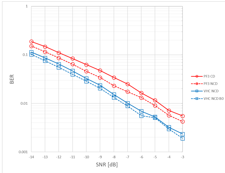
Figure 2: BER performance without intra-frequency hopping.
