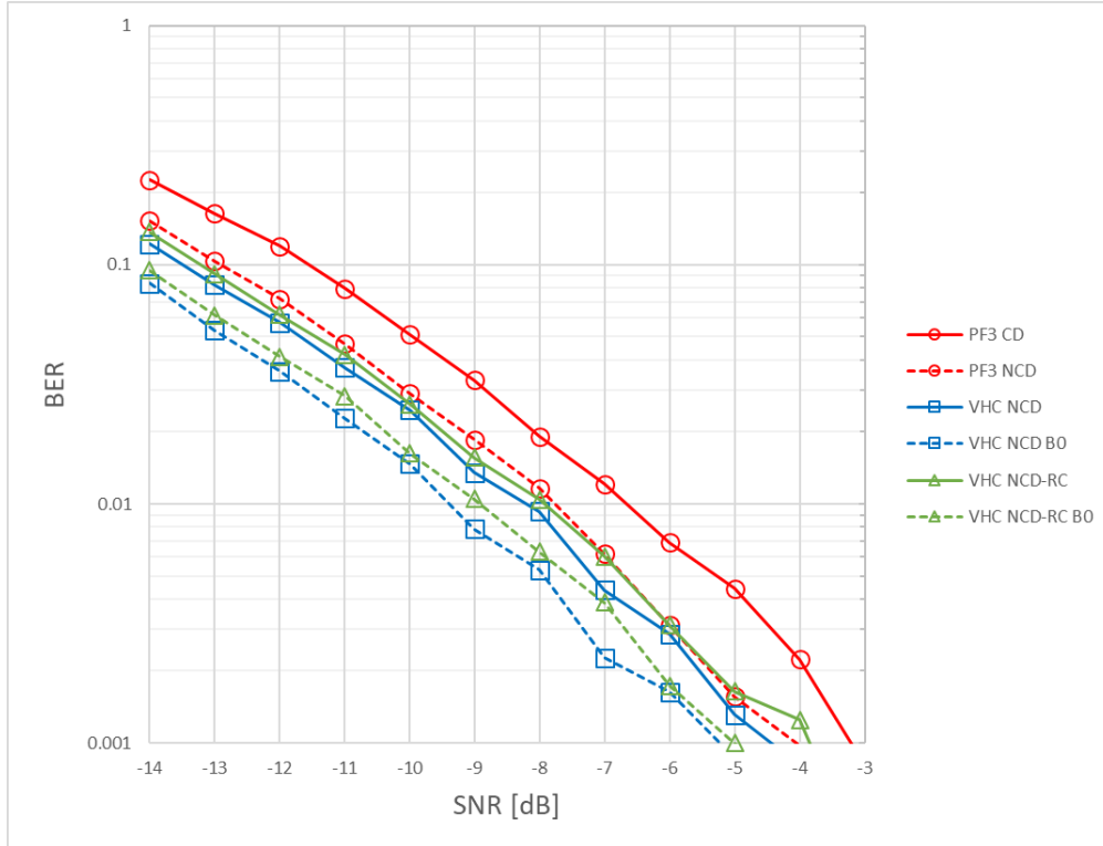
Figure 4: BER performance with intra frequency-hopping.
